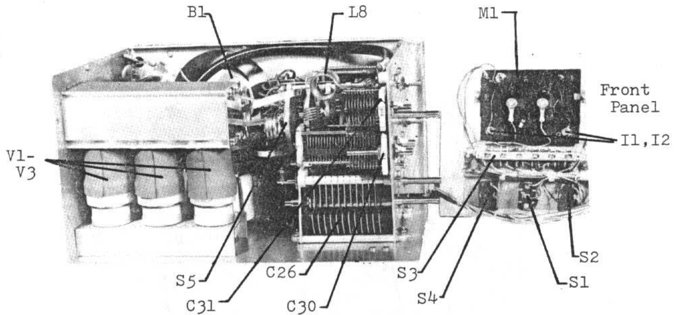
FIGURE 4 - Power Supply Side View, Cabinet Removed
