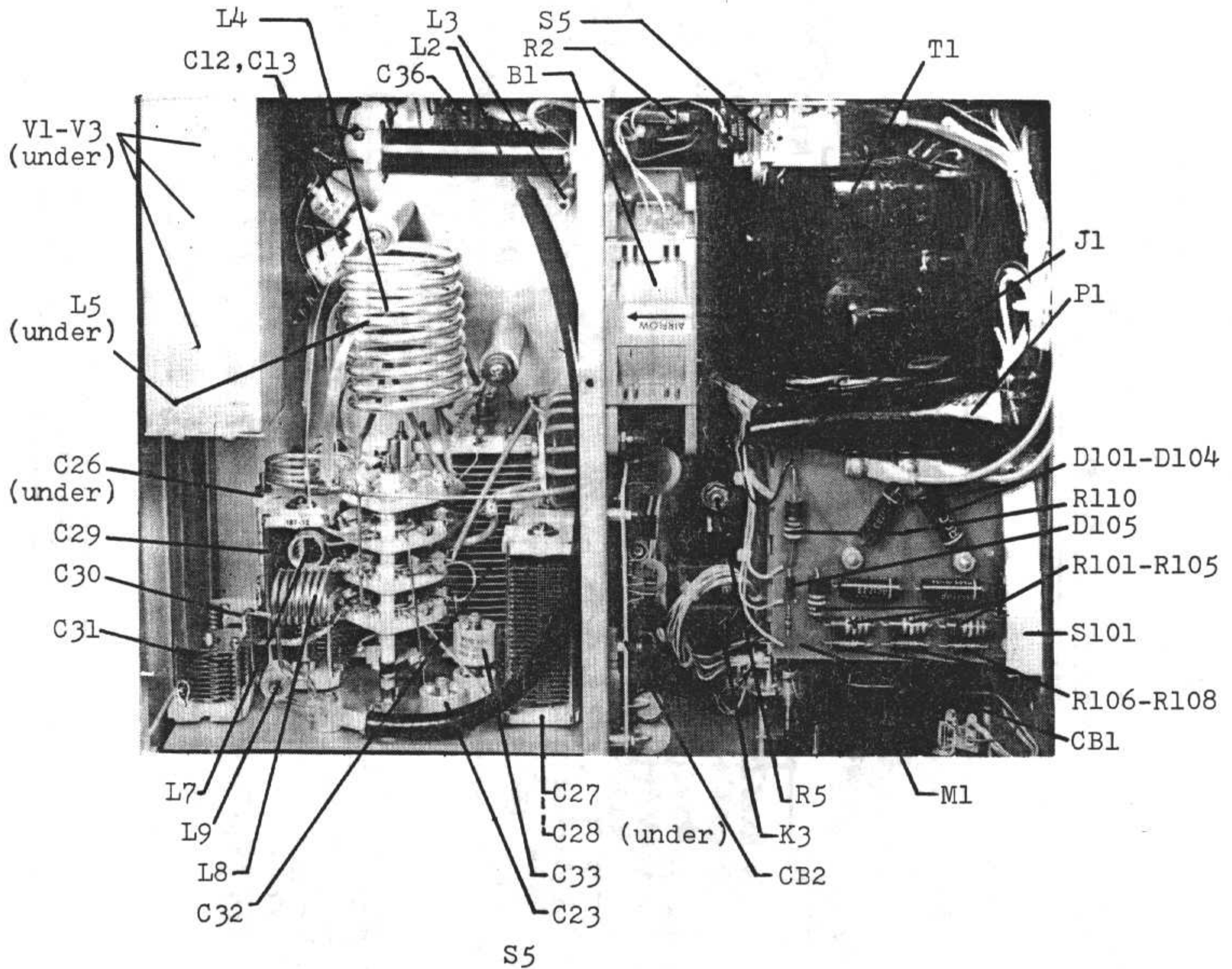
FIGURE 1 - Top View (Cover Removed)
